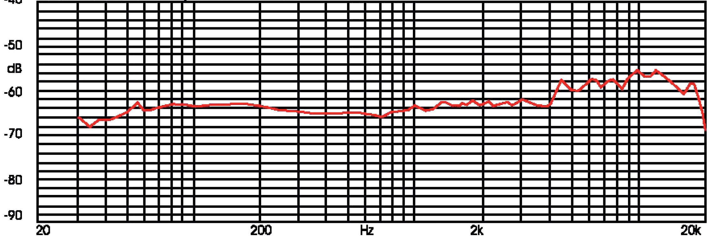
Frequency Response, Magn dB re 10.00V/Pa
