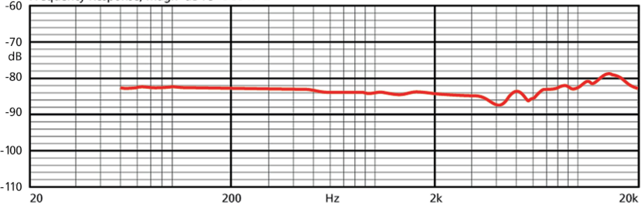
Frequency Response, Magn dB re 10.00 V/Pa
